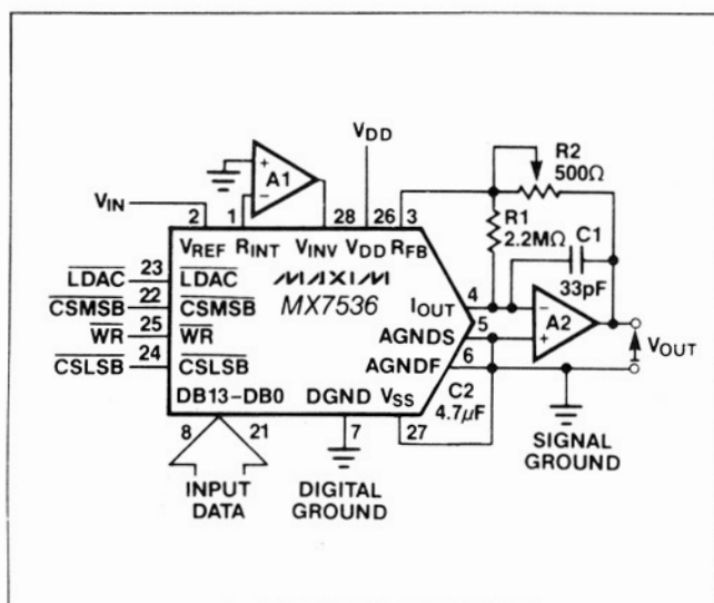
Figure 4. MX7536 Operation
