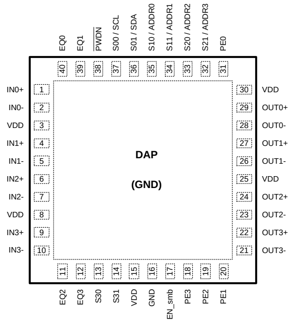
DS25CP104A / DS25CP114 Pin Diagram
