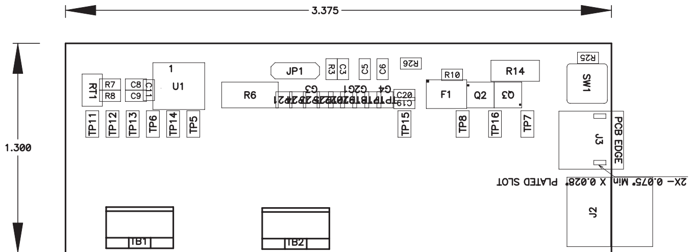
Figure 2. Top Assembly
