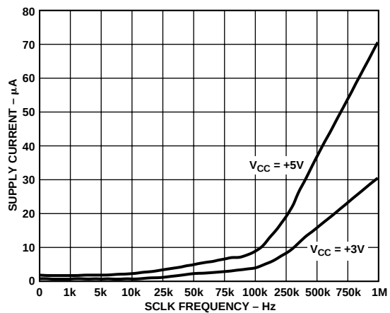
Figure 6. Standby Supply Current vs. Clock Frequency
