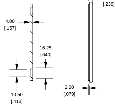
SECTION C-C Side of Slot
