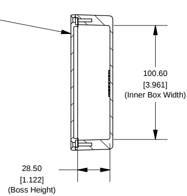
Top View Looking Inside Box
