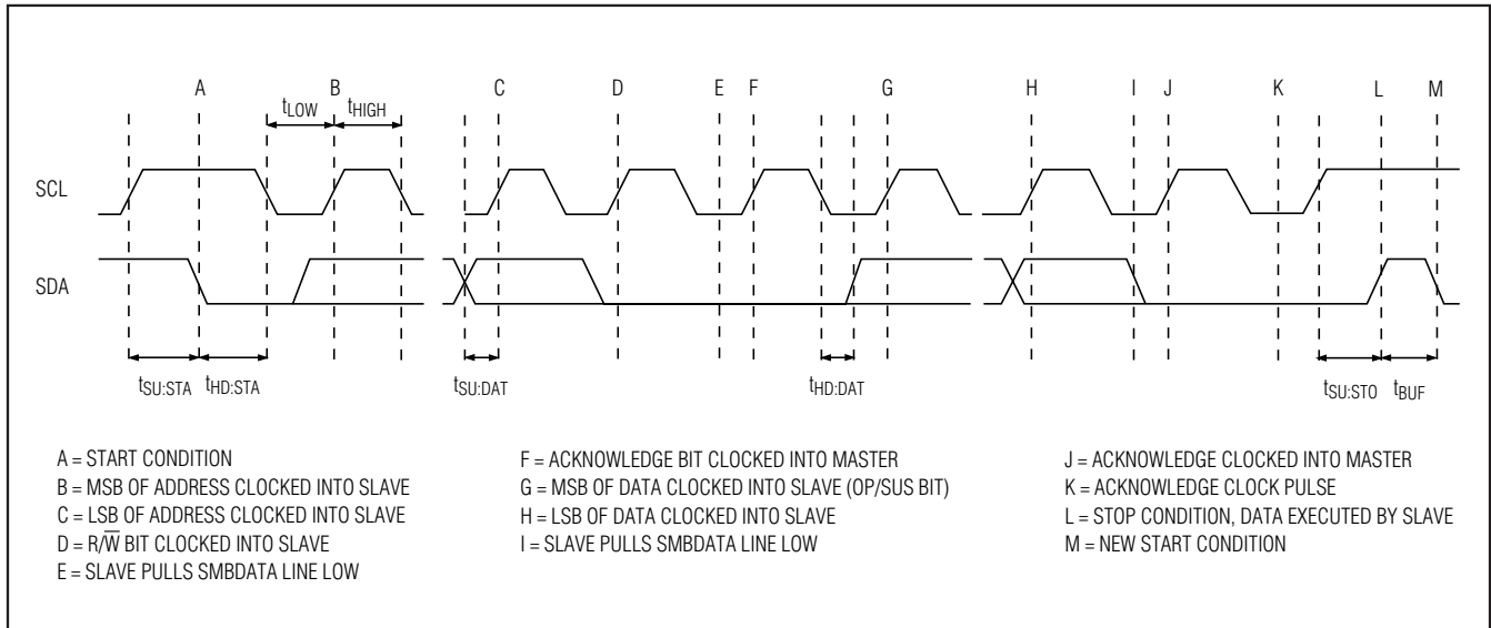
Figure 2. I²C-Compatible Serial-Interface Timing Diagram
