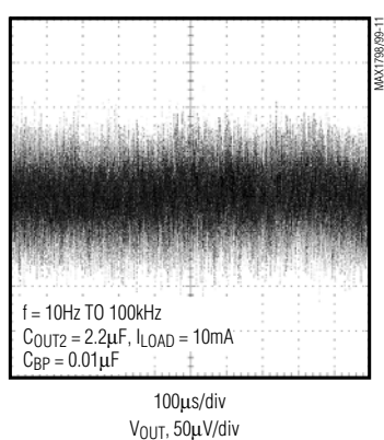
OUTPUT NOISE
