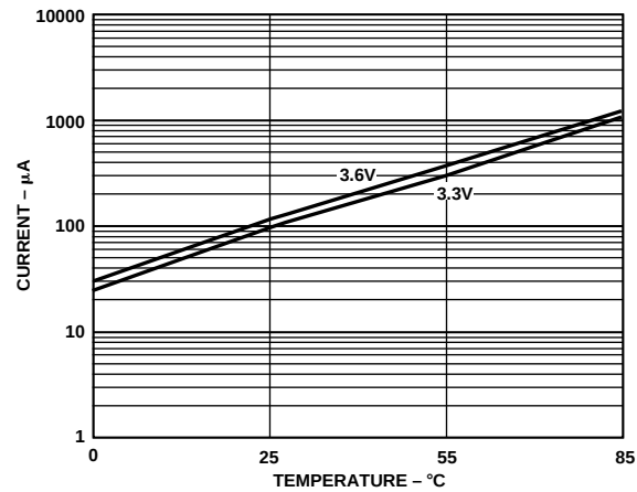
Figure 27. Rev 2.0 Power-Down Graph
