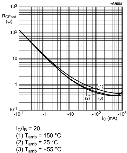
Fig. 11. TR2 (PNP): Equivalent on-resistance as a function of collector current; typical values
