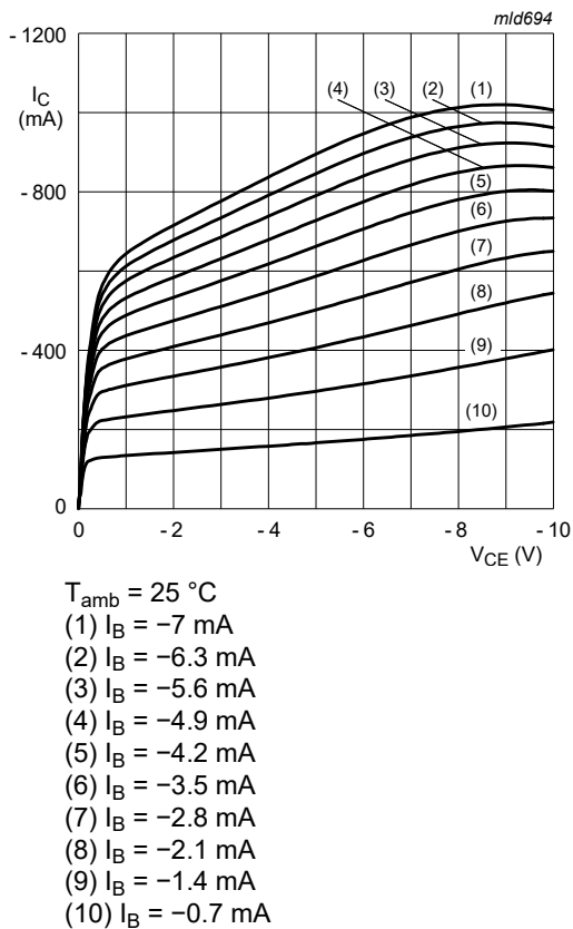
Fig. 12. TR2 (PNP): Collector current as a function of collector-emitter voltage; typical values
