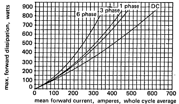
Figure 2 Dissipation / sink temperature v. mean forward current
