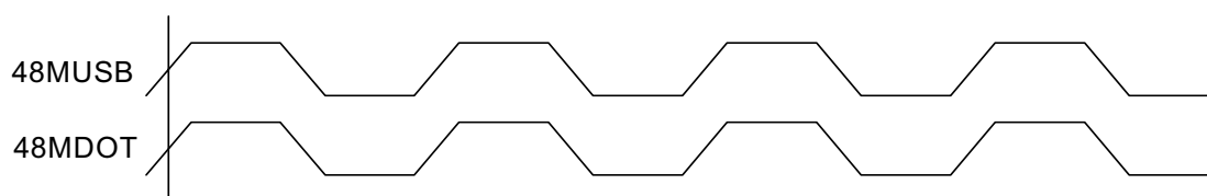
Figure 10. 48M_USB and 48M_DOT Phase Relationship
