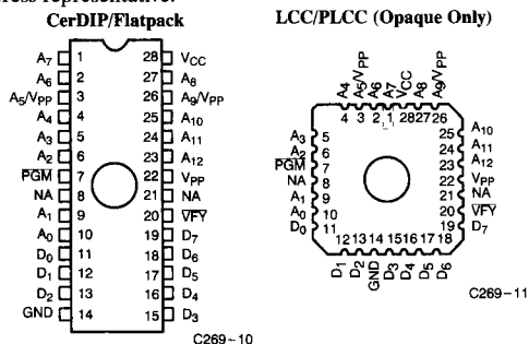
Figure 1. Programming Pinouts
