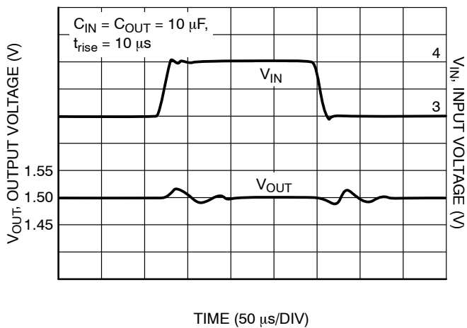
Figure 25. Line Transient ( V_{\text{out}} = 1.5 \text{ V} )
