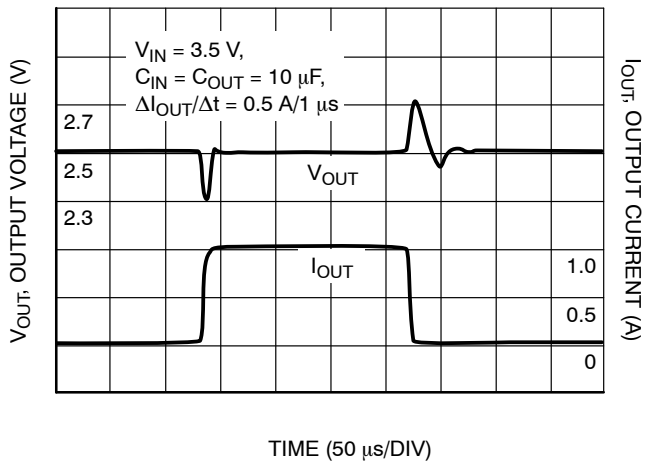
Figure 23. Load Transient ( V_{\text{out}} = 2.5 \text{ V} )
