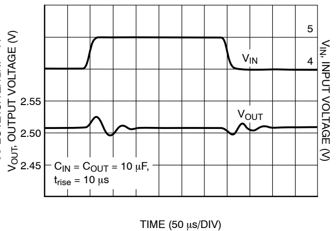
Figure 26. Line Transient ( V_{\text{out}} = 2.5 \text{ V} )
