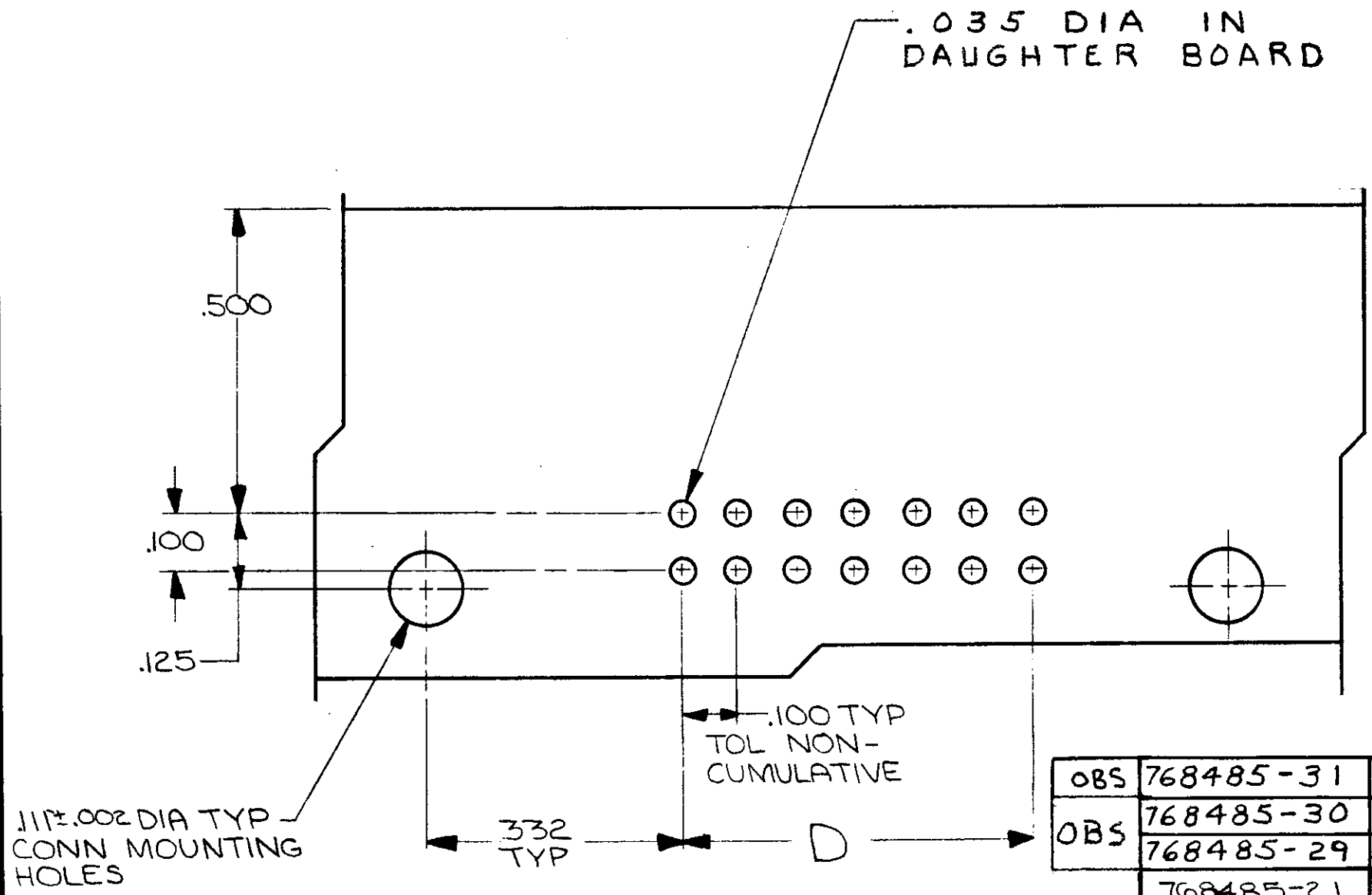
RECOMMENDED BOARD LAYOUT NOT TO SCALE
