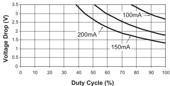
Device Duty Cycle vs. V_{DROP} V_{OUT} = 2.5V @ 85 degrees C
