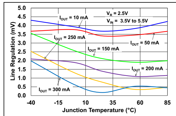
FIGURE 2-53: Line Regulation vs. Junction Temperature (MCP1812X, V_R = 2.5V ).
