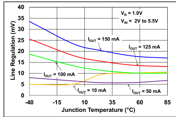
FIGURE 2-52: Line Regulation vs. Junction Temperature (MCP1811X, V_R = 1.0V ).
