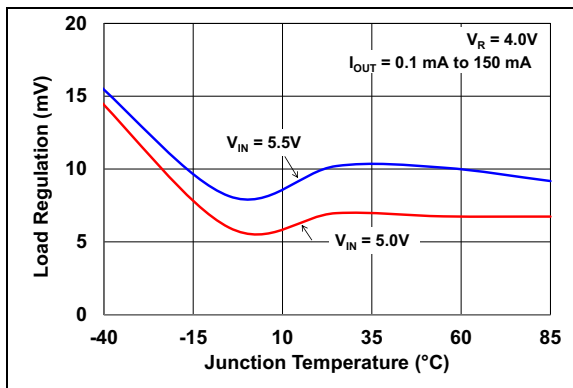
FIGURE 2-51: Load Regulation vs. Junction Temperature (MCP1811X, V_R = 4.0V ).
