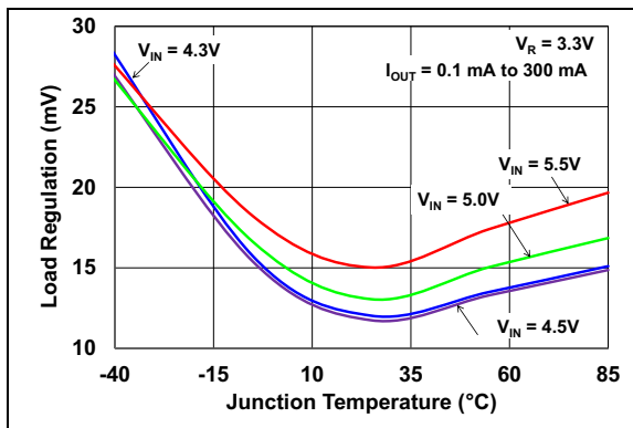
FIGURE 2-50: Load Regulation vs. Junction Temperature (MCP1812X, V_R = 3.3V ).
