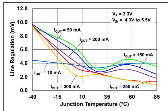
FIGURE 2-54: Line Regulation vs. Junction Temperature (MCP1812X, V_R = 3.3V ).
