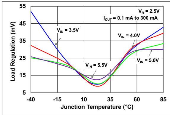
FIGURE 2-49: Load Regulation vs. Junction Temperature (MCP1812X, V_R = 2.5V ).
