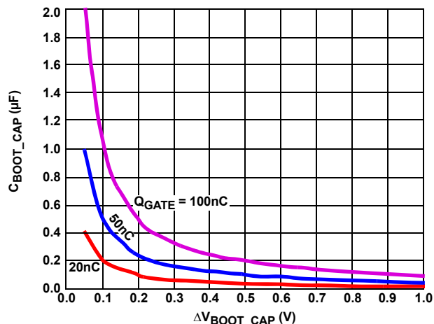
FIGURE 7. BOOTSTRAP CAPACITANCE vs. BOOT RIPLE VOLTAGE
