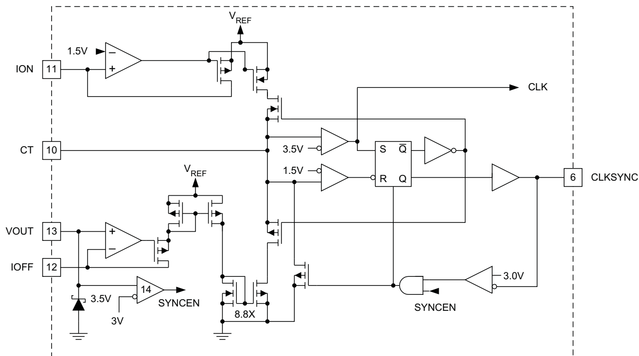
Figure 1. UCC3884 Oscillator
