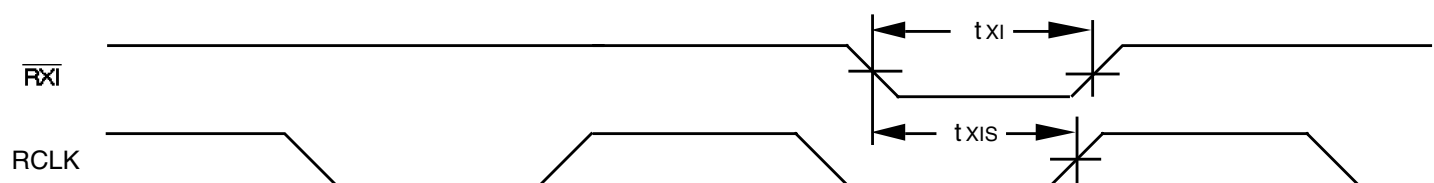
Figure 18. Read Expansion In Timing
