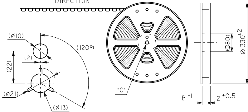
DETAIL "C"
