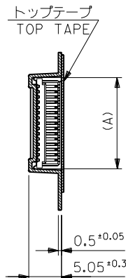
SECT. Y-Y
