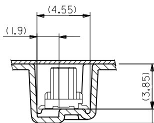
SECT. X-X (SCALE:5-1)
