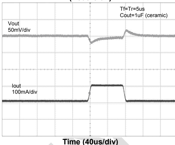
Output Load Transient Response (Vout=3.0V)
