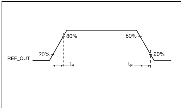
LVCOS Output Rise/Fall Time
