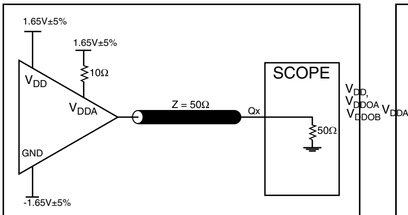
3.3V LVCMOS Output Load Test Circuit
