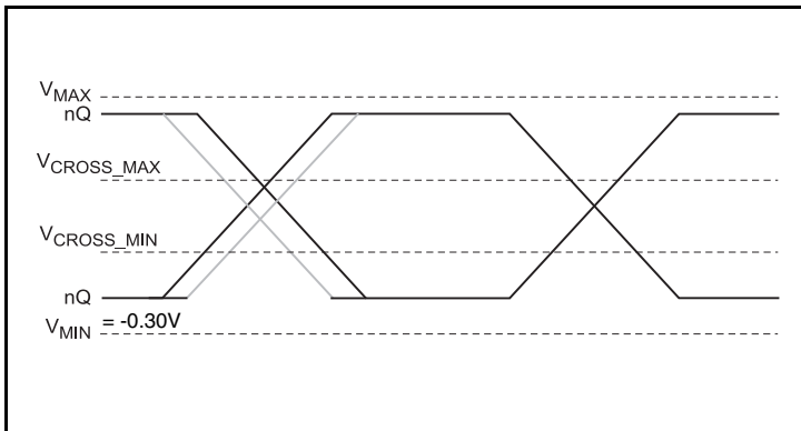
SE Measurement Points For Absolute Cross Point/Swing
