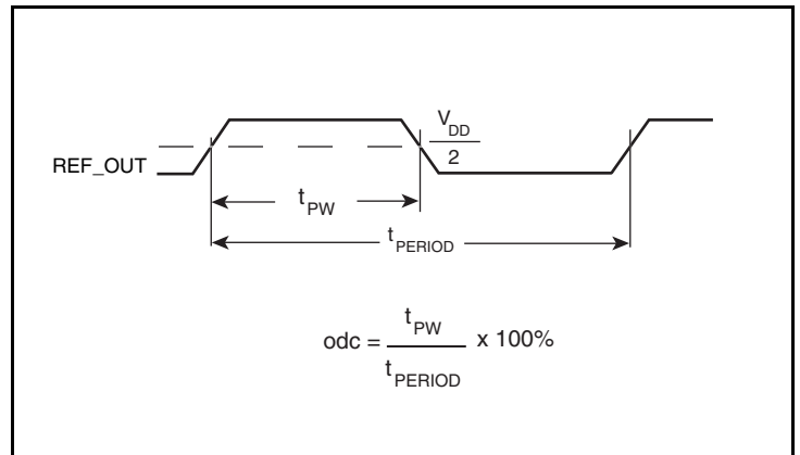
LVCOS Output Duty Cycle/Pulse Width/Period
