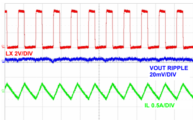
FIGURE 15. STEADY STATE OPERATION AT NO LOAD (PWM), (1 \mu\text{s}/\text{DIV} )
