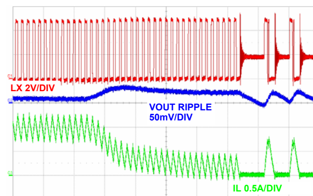
FIGURE 18. MODE TRANSITION CCM TO DCM, (5 \mu\text{s}/\text{DIV} )
