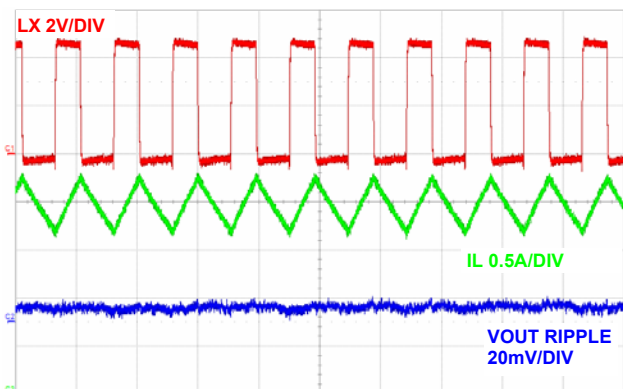
FIGURE 17. STEADY STATE OPERATION WITH FULL LOAD, (5 \mu\text{s}/\text{DIV} )
