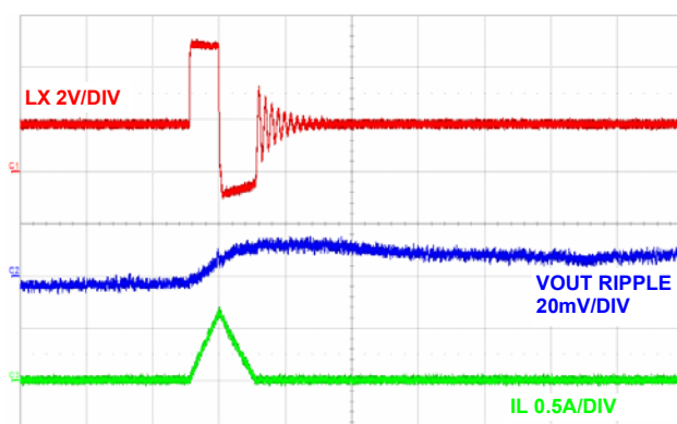
FIGURE 16. STEADY STATE OPERATION AT NO LOAD (PFM), (1 \mu\text{s}/\text{DIV} )
