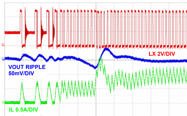
FIGURE 19. MODE TRANSITION DCM TO CCM, (50 \mu\text{s}/\text{DIV} )
