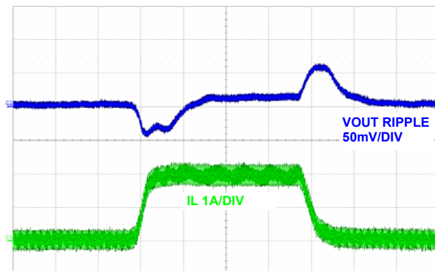
FIGURE 20. LOAD TRANSIENT (PWM), (50 \mu\text{s}/\text{DIV} )
