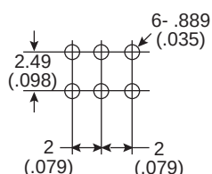
PCB Hole Detail
