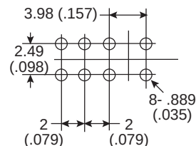
PCB Hole Detail
