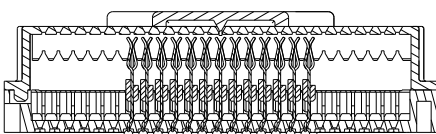
SECTION B-B
