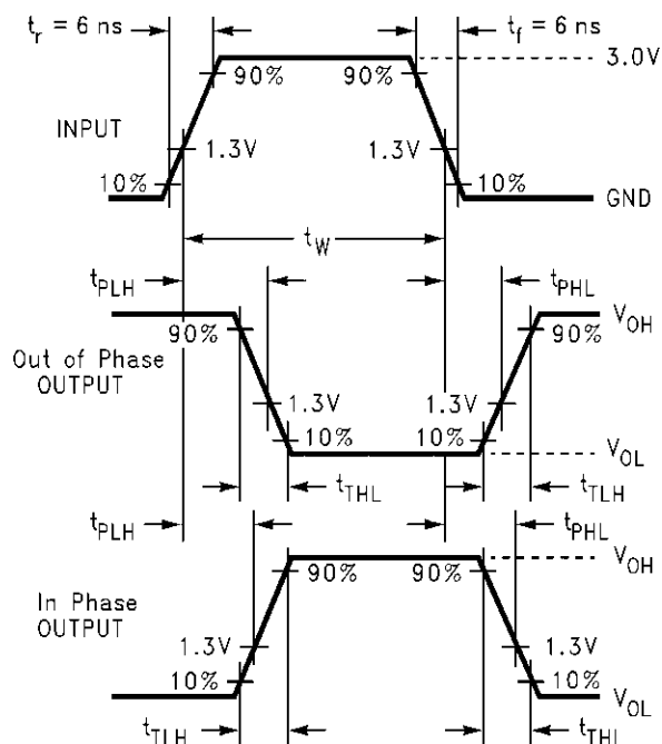
Figure 6. AC Waveforms
