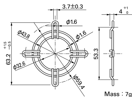
Outlet side
