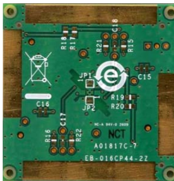
Figure 2. EB-O16CP44-2Z Circuit Side of PCB
