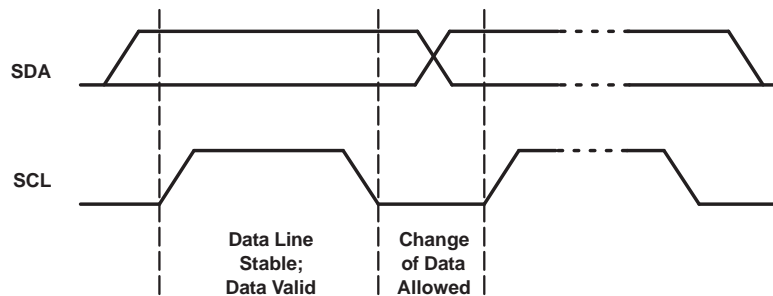
Figure 20. Bit Transfer
