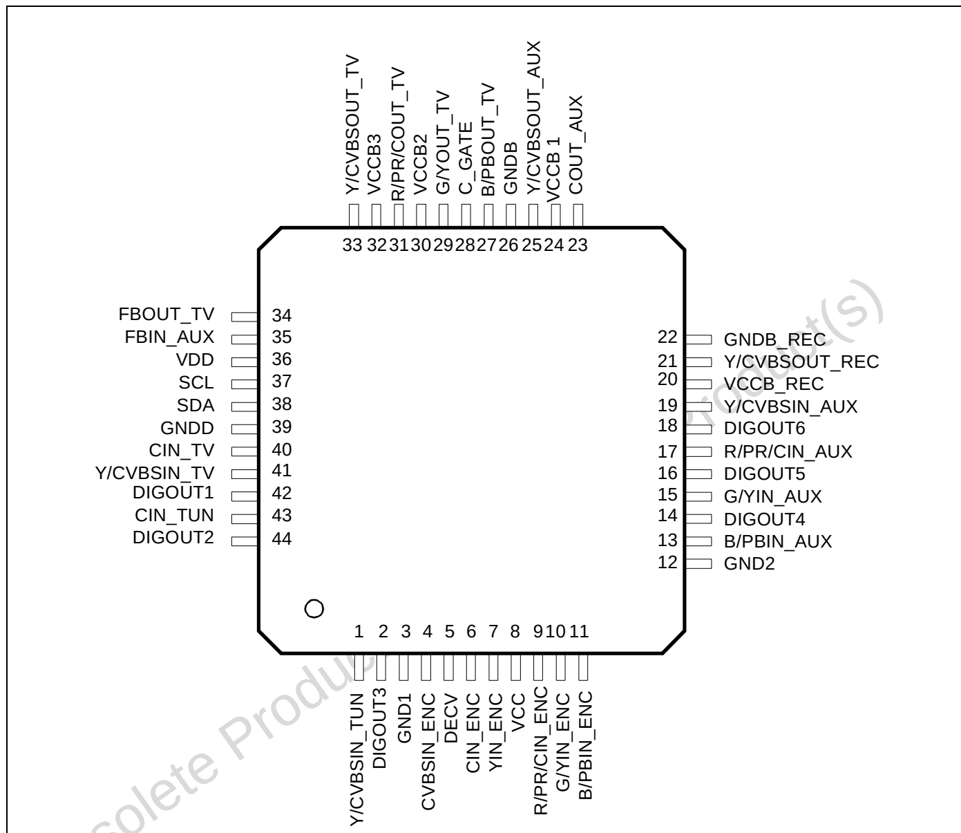
Figure 1: Pinout Diagram
