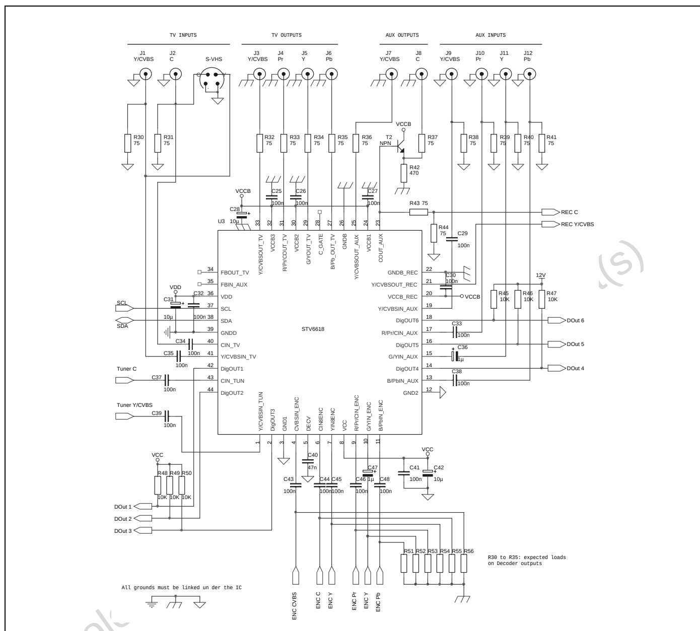
Figure 21: YPrPb Application
