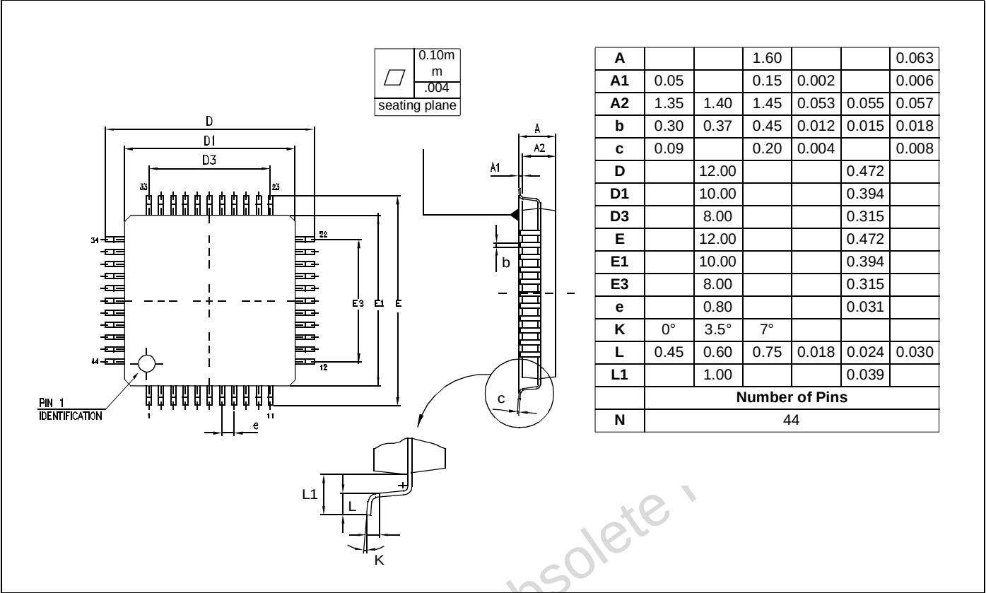
Figure 23: 44-Pin Thin Quad Flat Package
