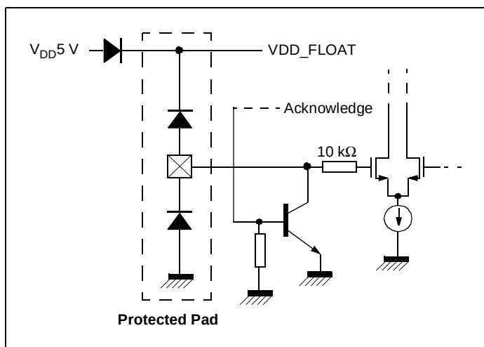
Figure 16: I²C Bus SDA I/O (Pin 38)
