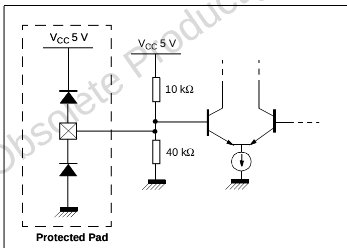
Figure 15: DECV (Pin 5)
