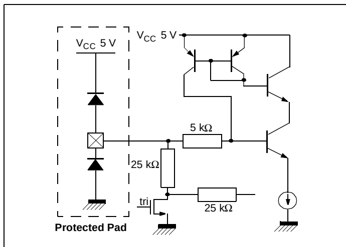
Figure 14: Average Clamped Video Inputs (Pins 6, 40 and 43)
