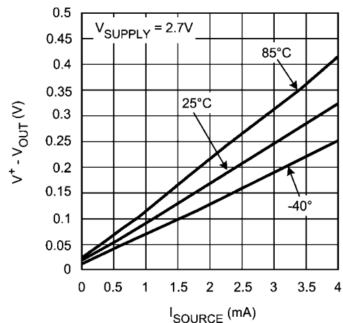
Output Positive Swing vs. I_{\text{SOURCE}}
