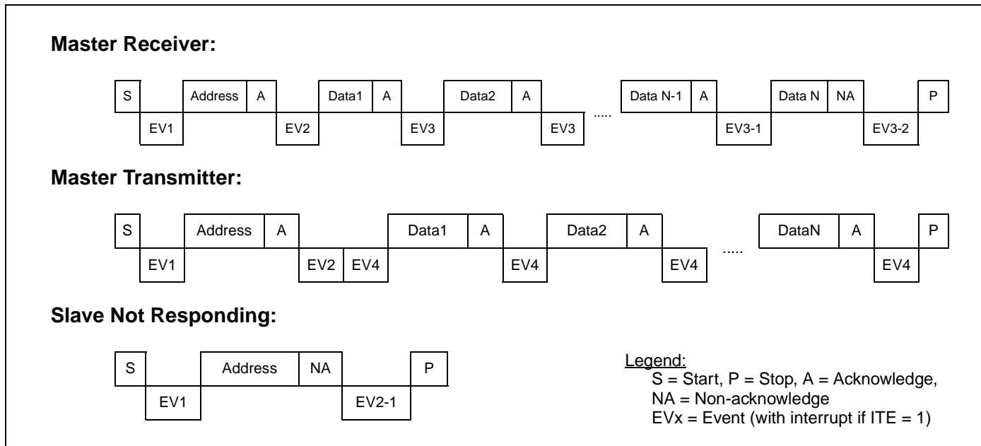
Figure 30: Transfer Sequencing
