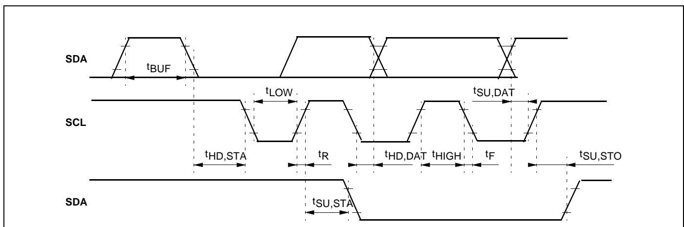
Figure 44: I 2 C Bus Timing
