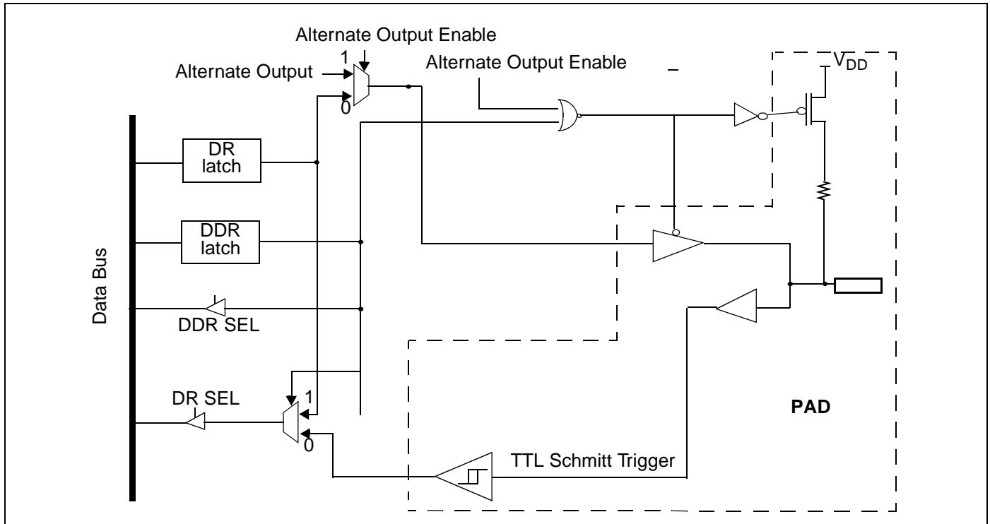
Figure 17: Port A [5:0]
