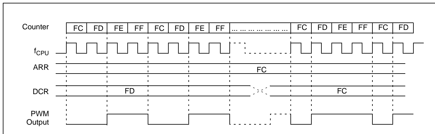
Figure 25: PWM Generation
