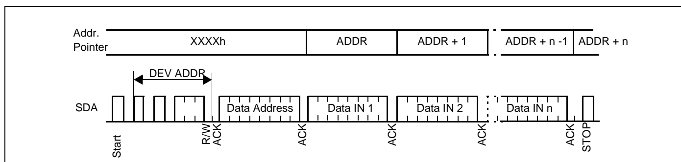
Figure 37: Write Sequence
