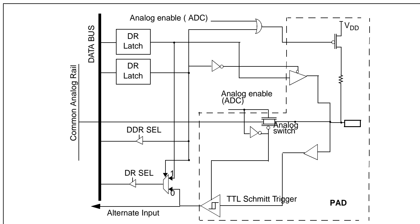
Figure 20: Port B [3]
