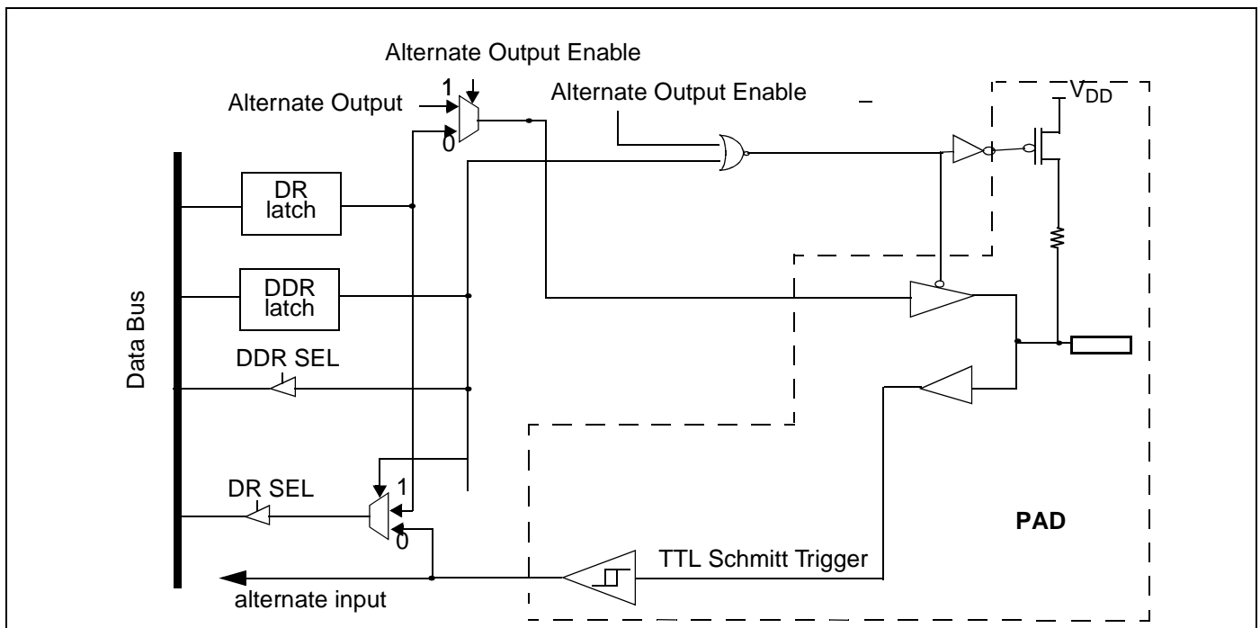
Figure 18: Port A [7:6]
