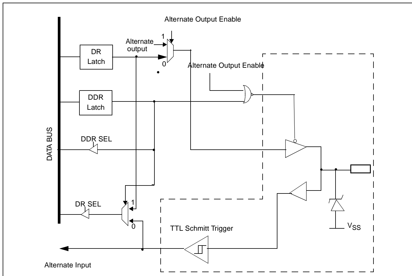
Figure 22: Port D
