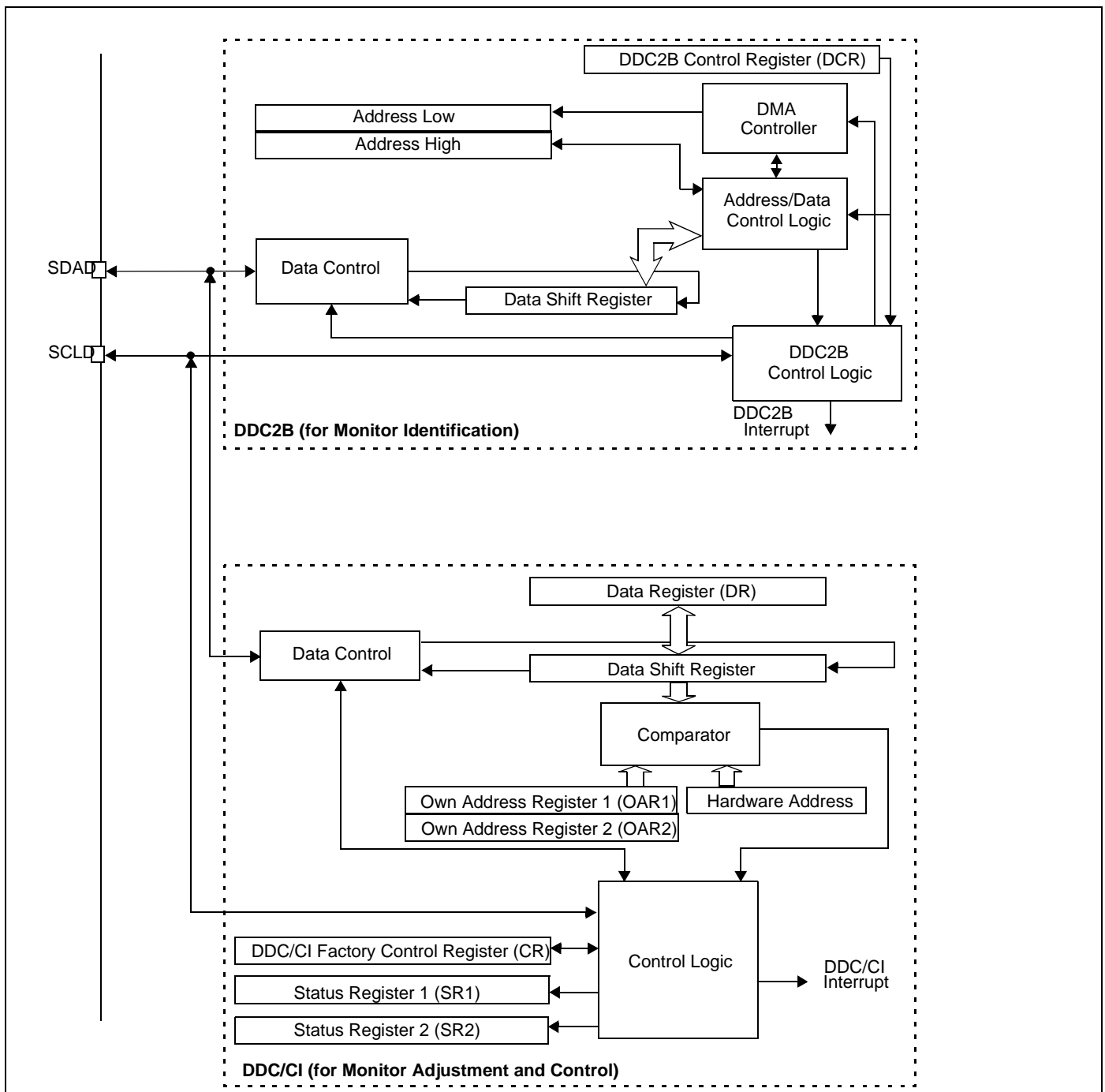
Figure 33: DDC Interface Block Diagram
