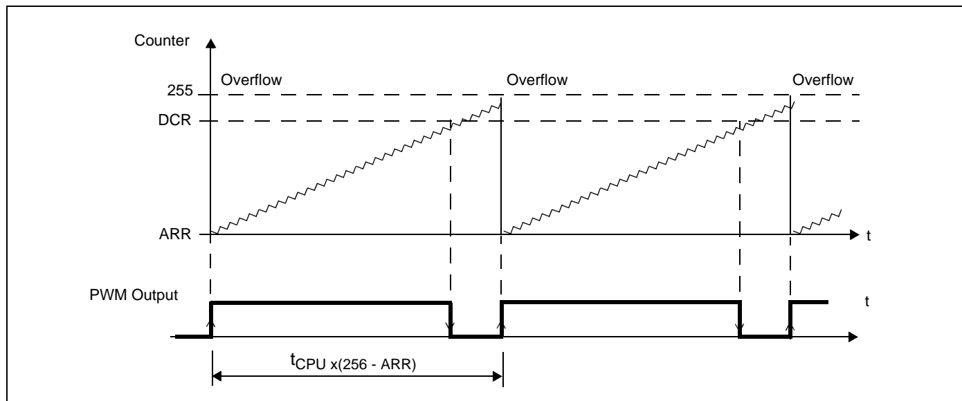
Figure 24: PWM Generation
