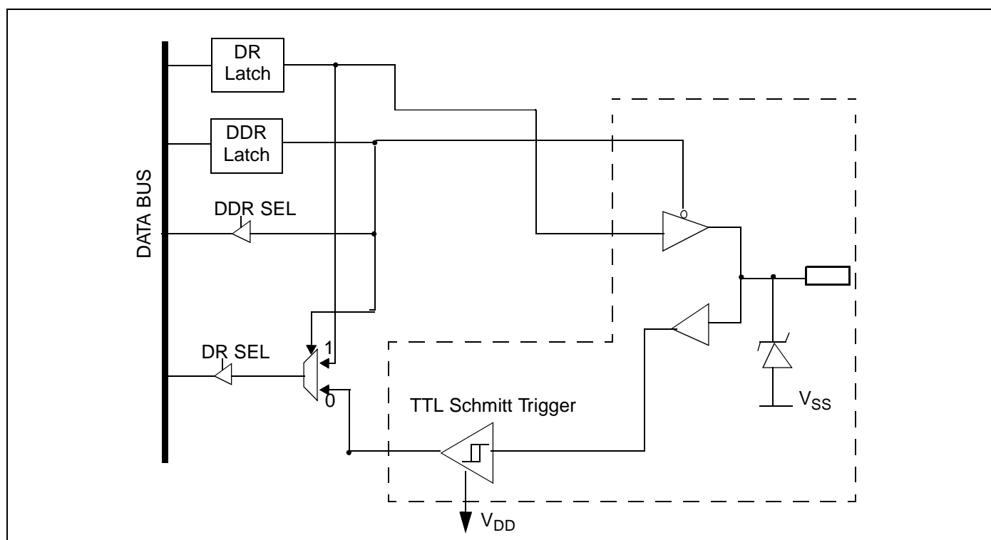
Figure 21: Port C
