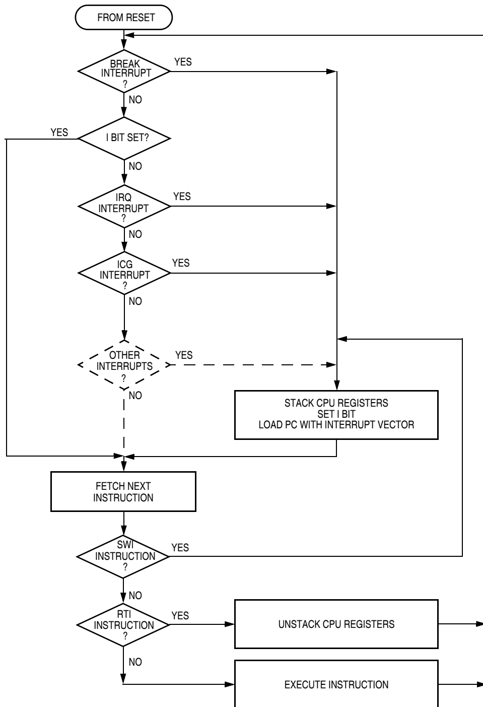
Figure 13-6. Interrupt Processing
