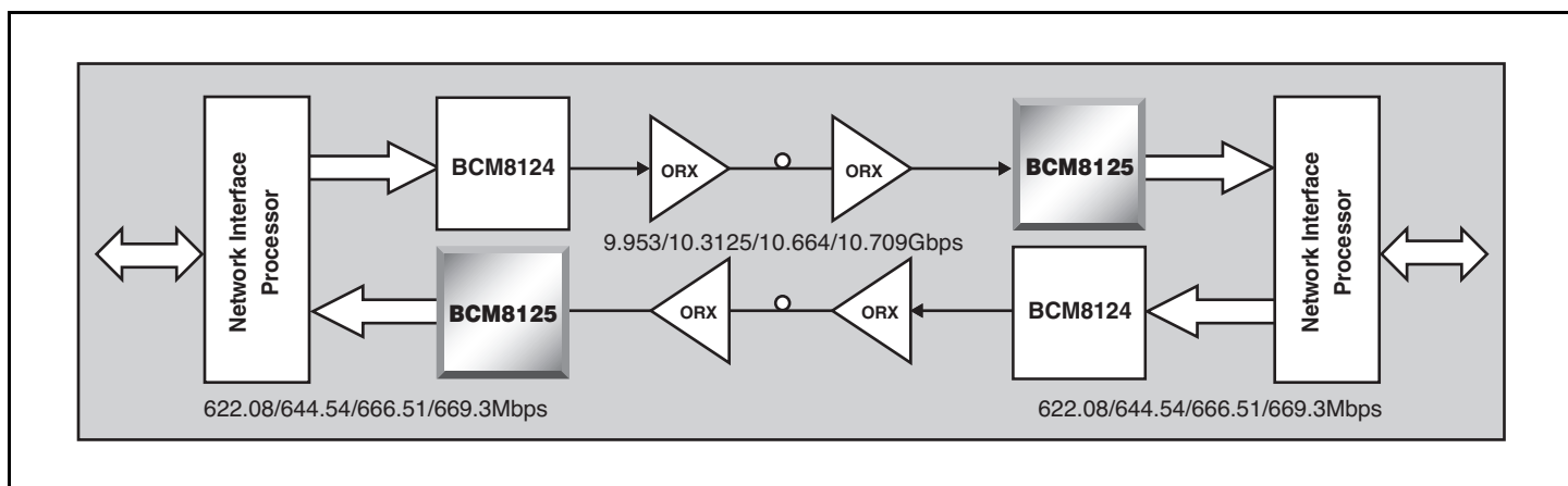
BCM8125 Application Diagram
