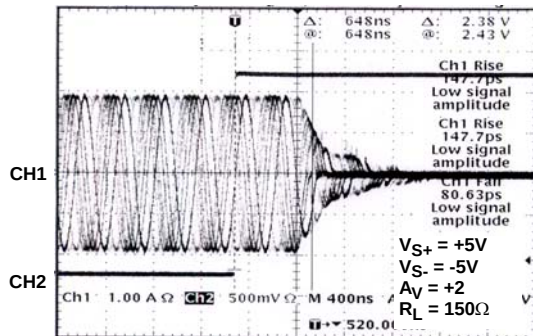
FIGURE 15. TURN-OFF DELAY, V_{IN} = 100\text{mV}_{p-p}
