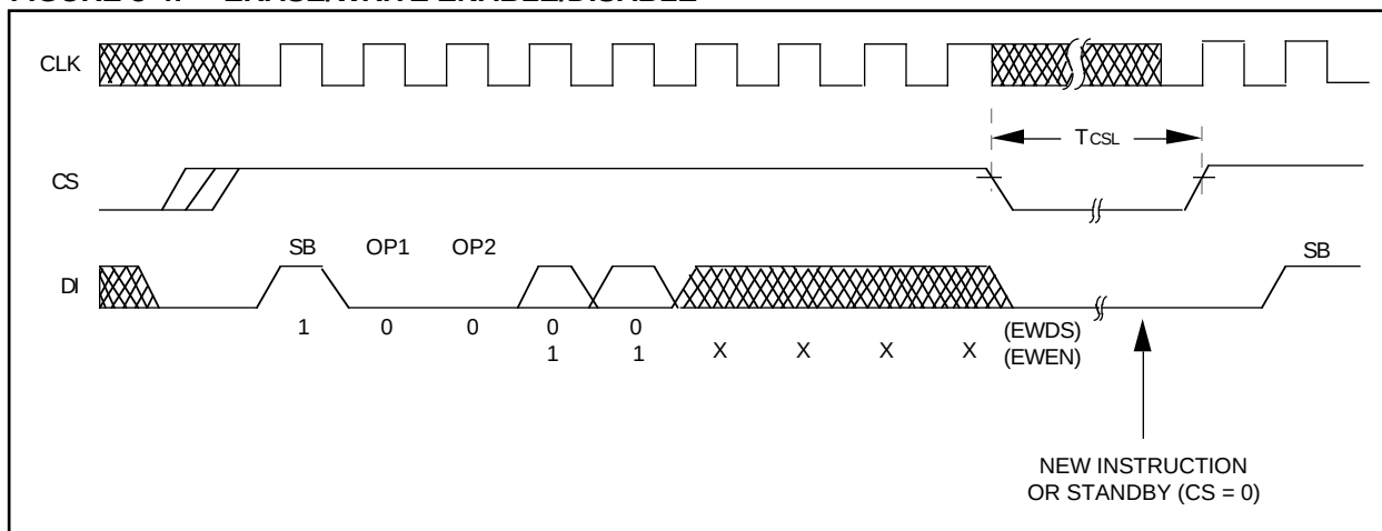
FIGURE 3-4: ERASE/WRITE ENABLE/DISABLE
