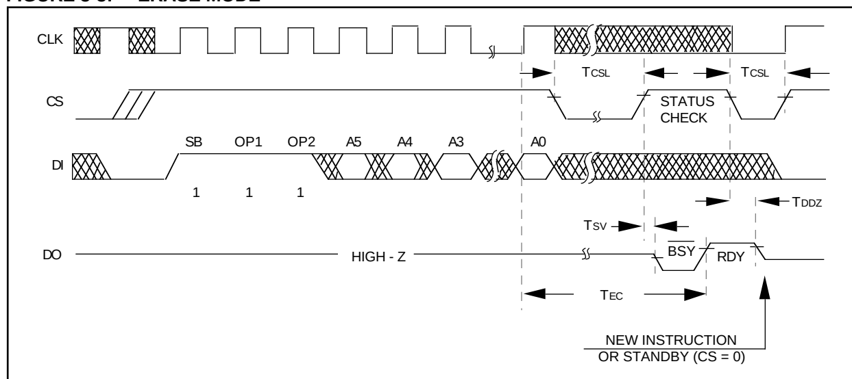
FIGURE 3-3: ERASE MODE
