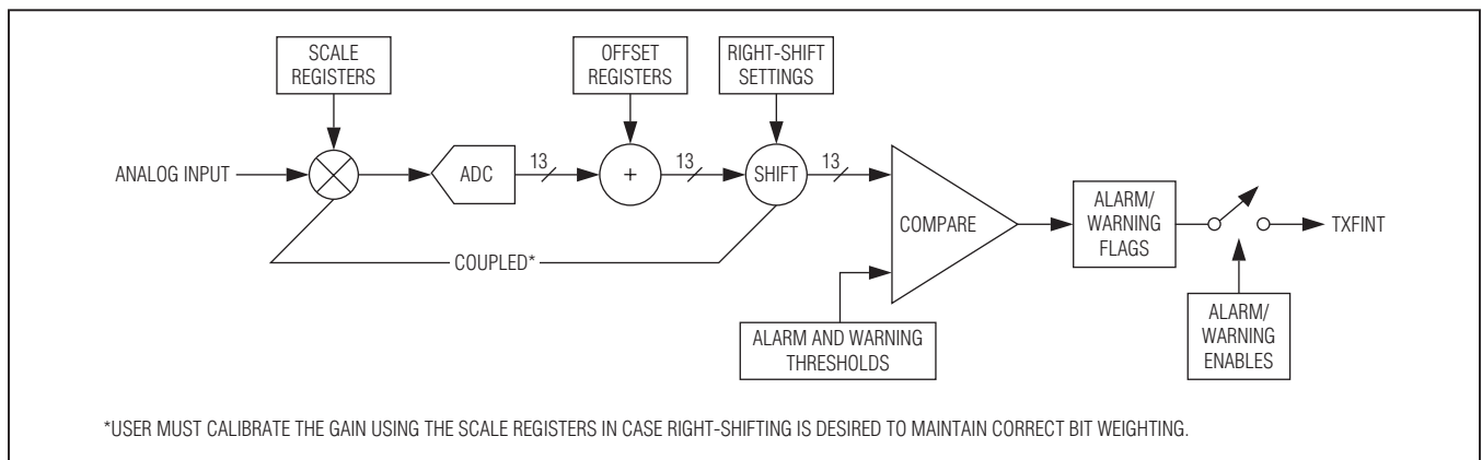
Figure 1. ADC Channel
