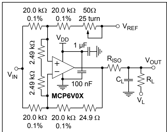
The circuit in Figure 1-7 tests the op amp input's dynamic behavior (i.e., IMD , t_{STR} , t_{STL} and t_{ODR} ). The potentiometer balances the resistor network ( V_{OUT} should equal V_{REF} at DC). The op amp's common mode input voltage is V_{CM} = V_{IN}/2 . The error at the input ( V_{ERR} ) appears at V_{OUT} with a noise gain of 10 V/V.
