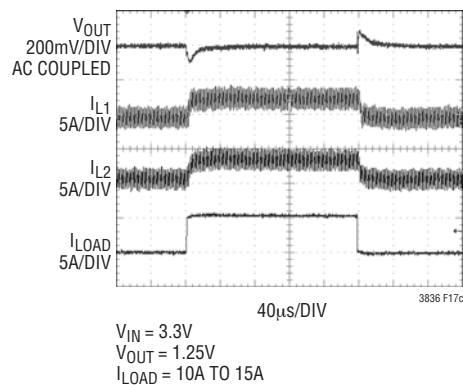
Figure 17c. Load Step
