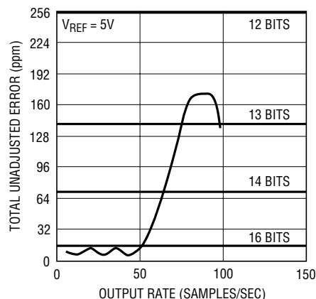
Figure 7. Total Error vs Output Rate ( V_{BFF} = 5V )
