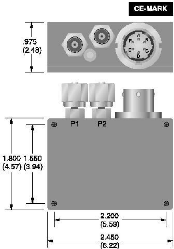
Figure 9.1—PPT Case Outline
