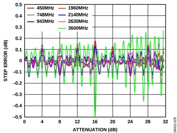
Figure 29. DSA: Step Error vs. Attenuation
