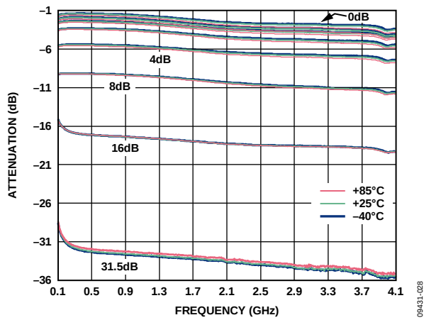
Figure 28. DSA: Attenuation vs. Frequency and Temperature
