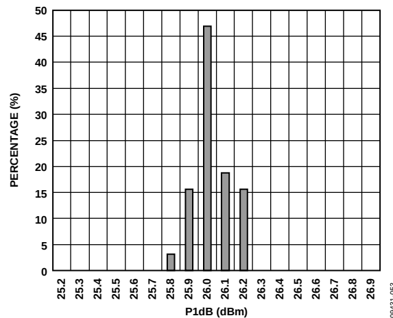
Figure 55. AMP2: P1dB Distribution at 2140 MHz
