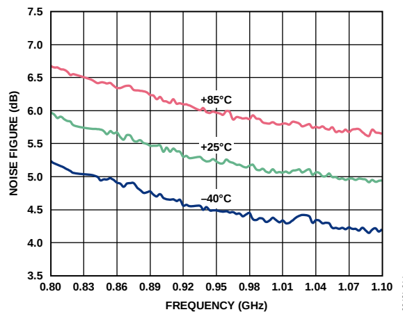
Figure 14. AMP2-943 MHz: Noise Figure vs. Frequency and Temperature
