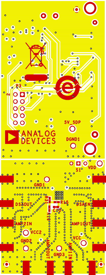
Figure 78. Evaluation Board Layout—Bottom
