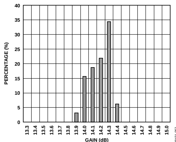
Figure 54. AMP2: Gain Distribution at 2140 MHz
