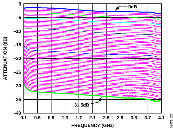
Figure 27. DSA: Attenuation vs. Frequency
