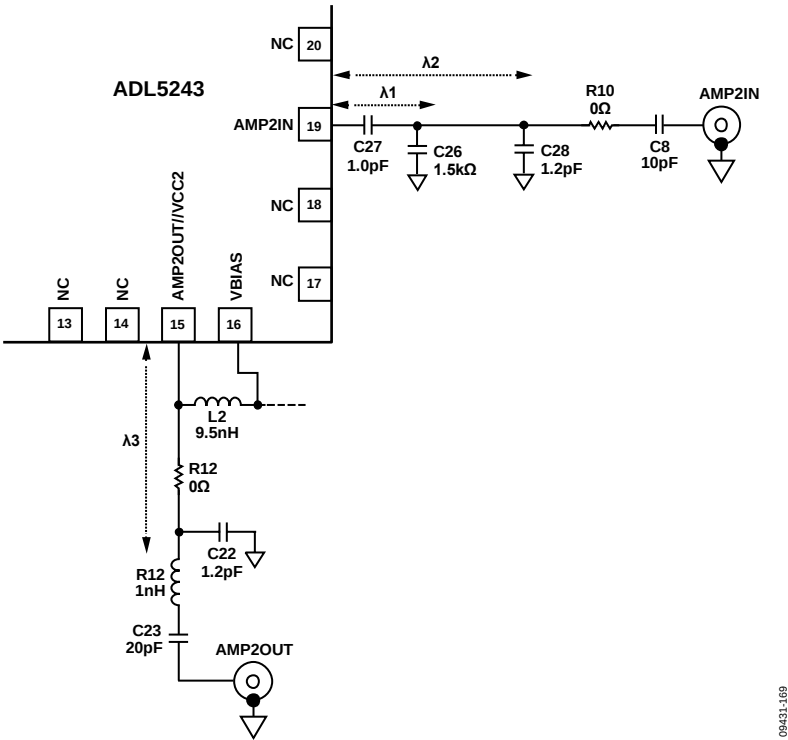
Figure 69. AMP2: Matching Circuit at 3600 MHz
