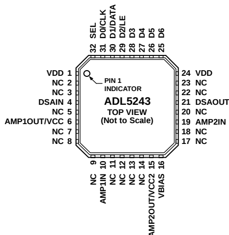
Figure 2. Pin Configuration
