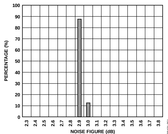
Figure 53. AMP1: Noise Figure Distribution at 2140 MHz
