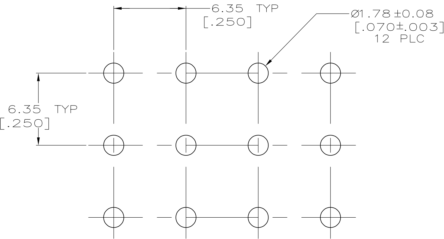
RECOMMENDED MOUNTING HOLE PATTERN FOR A 3.18 [.125] THK P.C. BOARD
