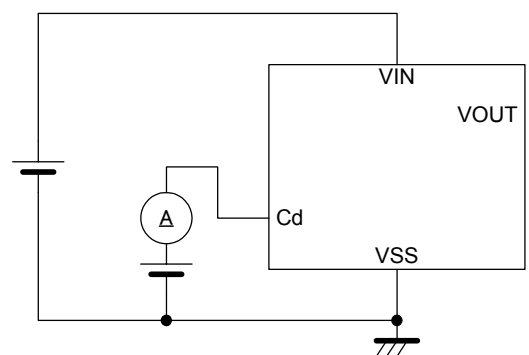
Circuit 4
