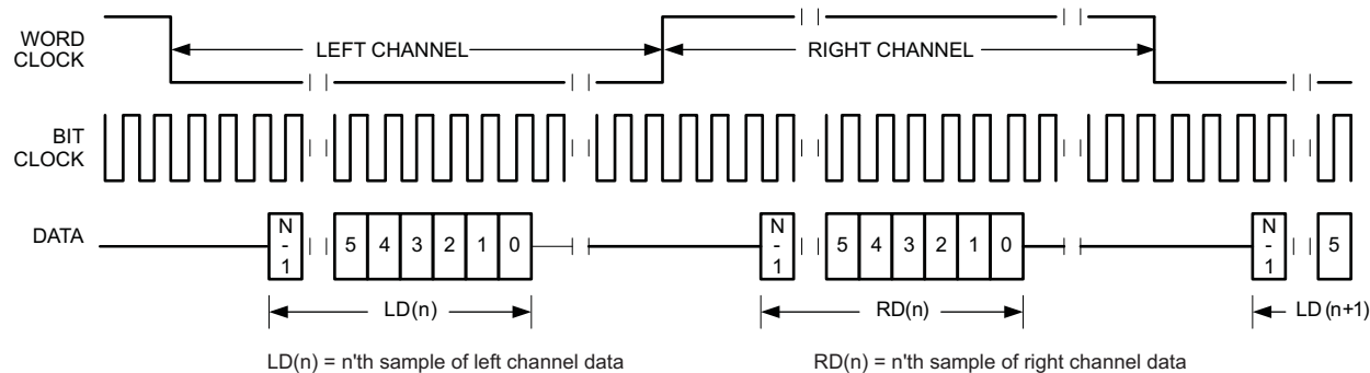
Figure 7-44. Timing Diagram for I²S Mode With Offset = 2
