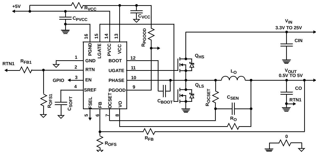
FIGURE 1. ISL95870 APPLICATION SCHEMATIC WITH ONE OUTPUT VOLTAGE SETPOINT AND DCR CURRENT SENSE
