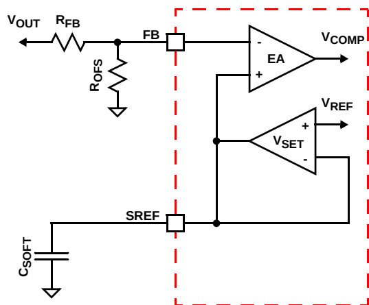
FIGURE 9. ISL95870 VOLTAGE PROGRAMMING CIRCUIT
