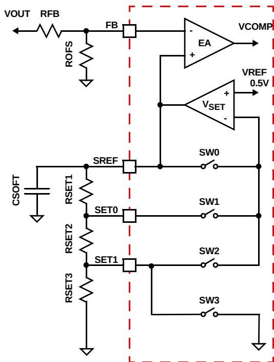
FIGURE 10. ISL95870A VOLTAGE PROGRAMMING CIRCUIT
