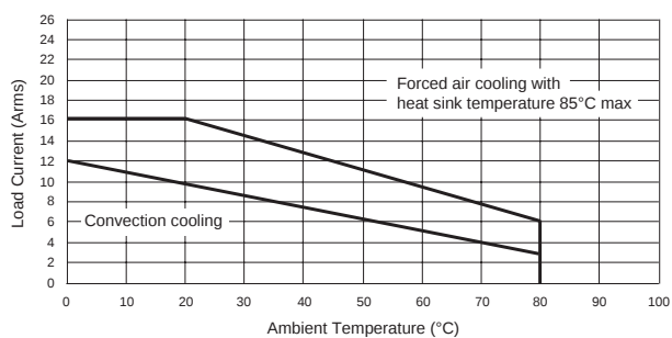
Figure 13a — LS24D16X-HS1 relays
