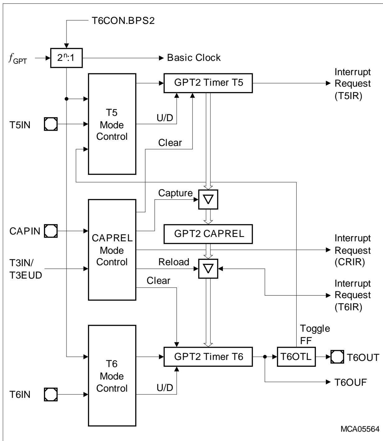
Figure 3-6 Block Diagram of GPT2
