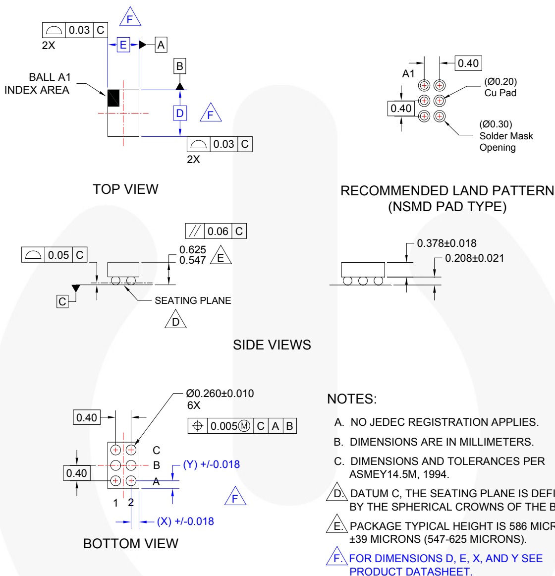
Figure 42. 6-Bump WLCSP, 0.4mm Pitch
