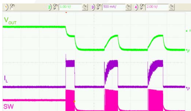
Figure 35. Over-Current Fault Response, R_{LOAD} = 1\Omega , 50\mu s/div.
