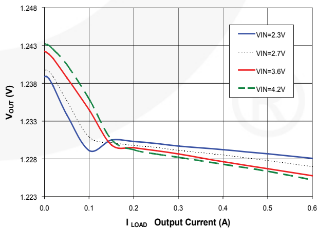
Figure 10. 1.233V OUT Load Regulation vs. Input Supply
