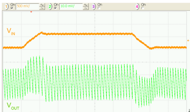
Figure 20. Line Transient 3.3V_{IN} to 3.9V_{IN} , 50mA Load, 10\mu s/div.
