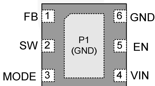
Figure 4. UMLP, Leads Facing Down
