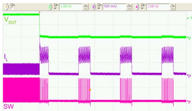
Figure 33. Metallic Short Applied at V_{OUT} , 50\mu s/div.
