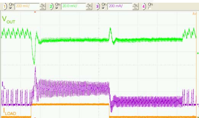
Figure 25. Load Transient 50 to 250mA, 2.5V_{IN}
