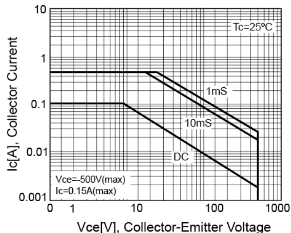
Figure 5. Safety Operation Area
