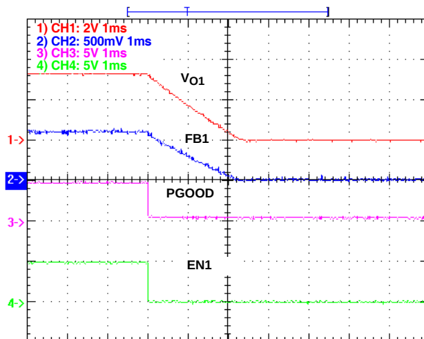
FIGURE 10. ENABLE CONTROL, EN1 = \text{LOW} , V_{IN} = 12V , V_{O1} = 3.3V , I_{O1} = 5A
