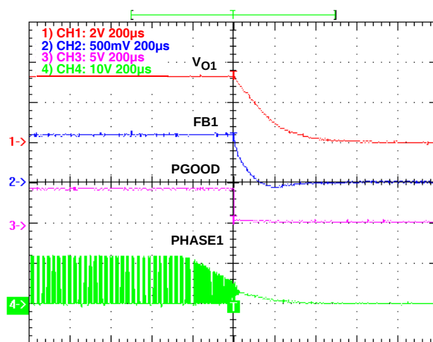
FIGURE 8. POWER-OFF, V_{IN} = 12V , I_{O1} = 5A , V_{O1} = 3.3V
