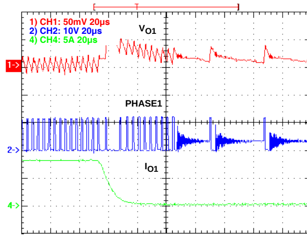
FIGURE 16. LOAD RELEASE RESPONSE, V_{IN} = 12V , V_{O1} = 3.3V , I_{O1} = 0.1A/8.1A @ 2.5A/μs
