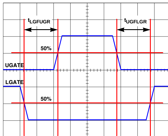
FIGURE 25. LGATE AND UGATE DEAD-TIME
