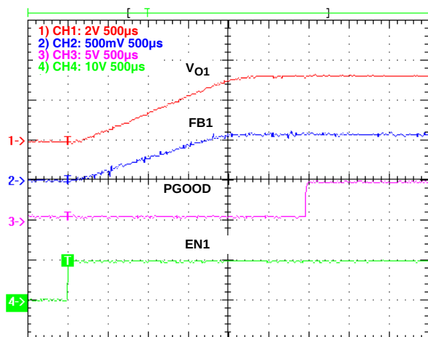
FIGURE 9. ENABLE CONTROL, EN1 = \text{HIGH} , V_{IN} = 12V , V_{O1} = 3.3V , I_{O1} = 5A
